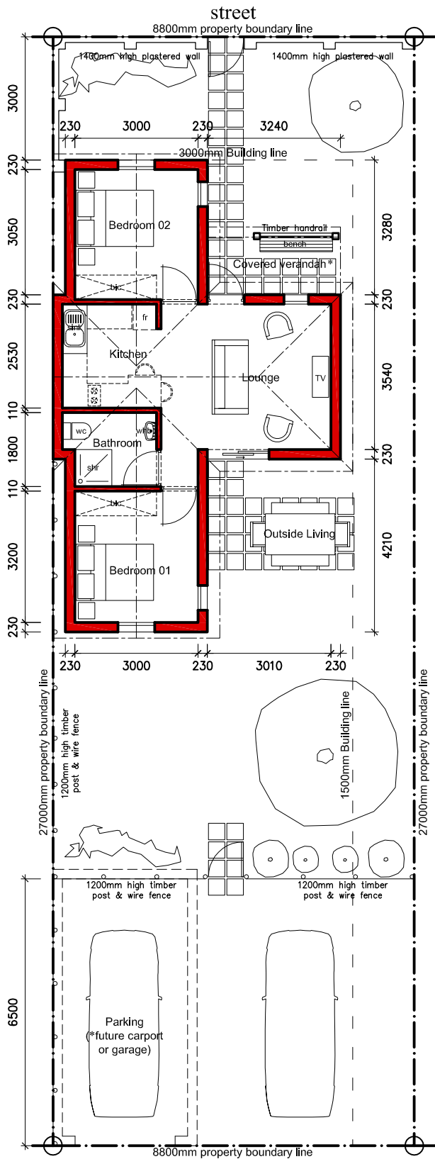
rear lane GROUND FLOOR
